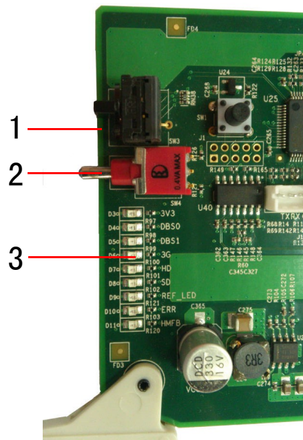
Figure 4-1 The Switches and LED Lights of HUC6830N/HUC6830NS
