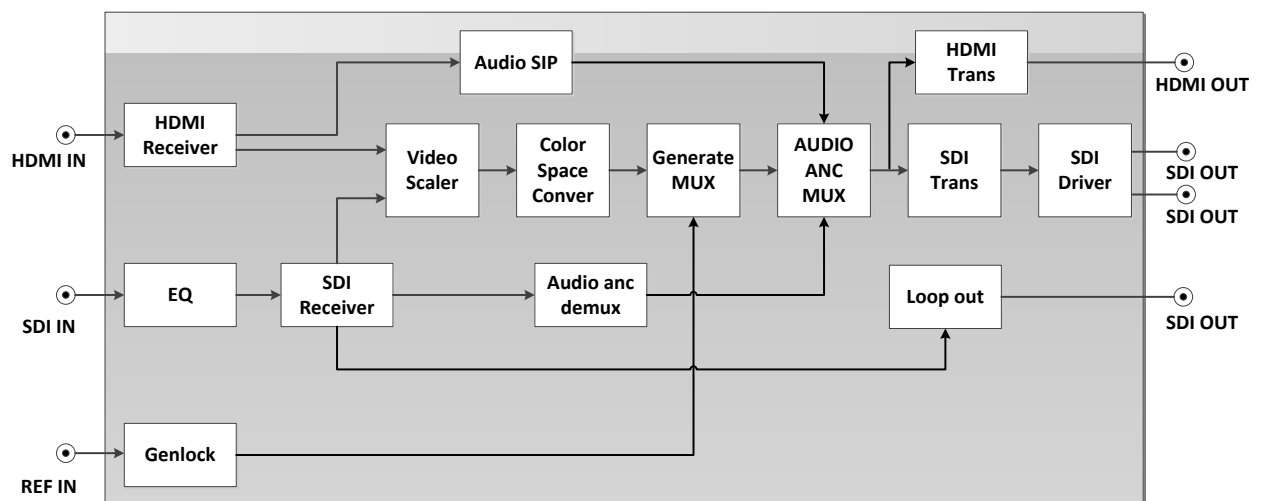
Figure 1-2 The Signal Flow Chart of HUC6830N/HUC6830NS
