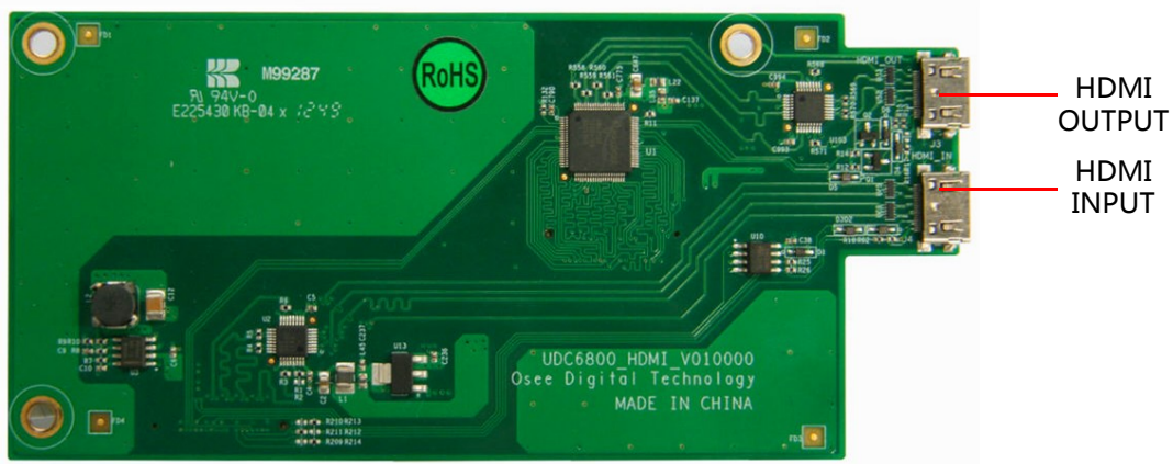
Figure 5-5 HDMI Input/Output Module
