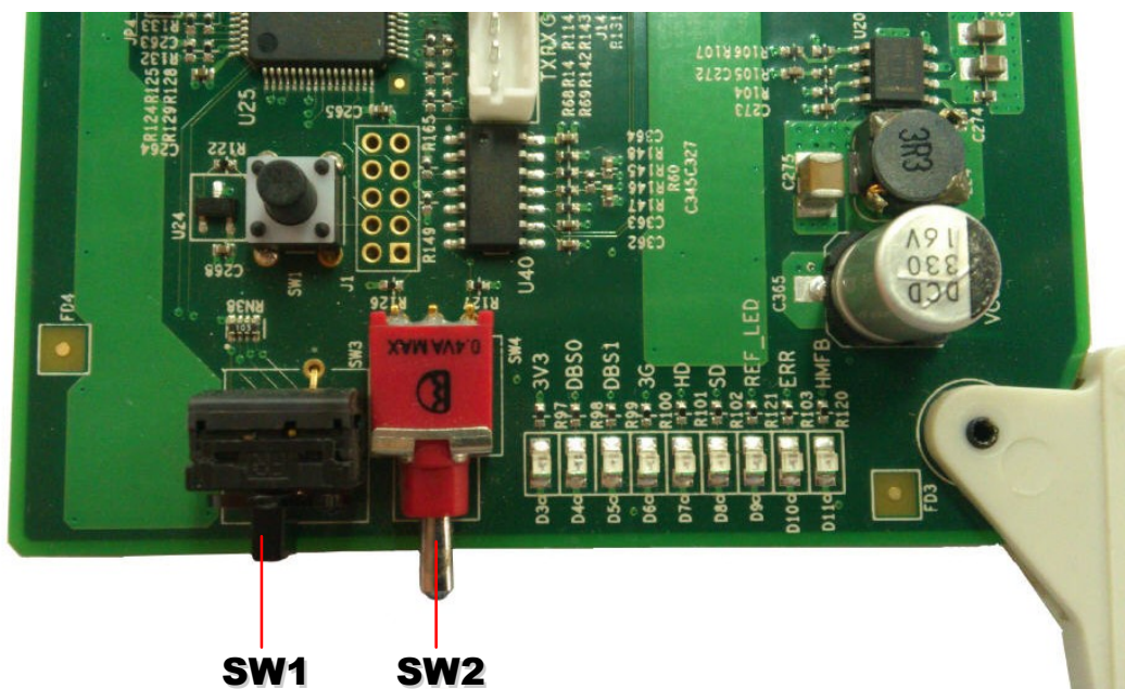
Figure 5-1 The Position of Control Switches
