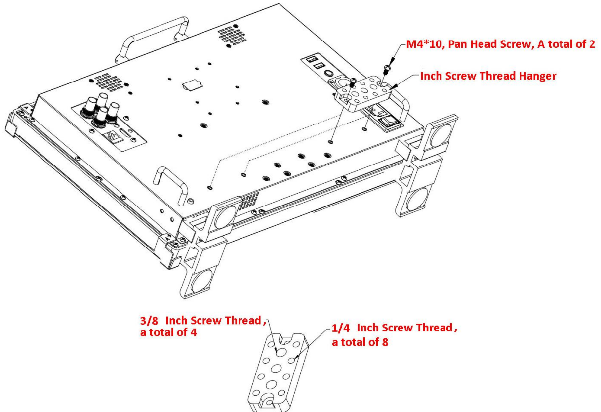
Figure 5.2-14 Inch Screw Thread Hanger
