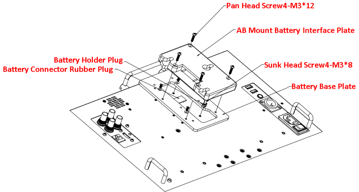
Figure 5.2-3 AB-mount Battery Plate in Portrait
