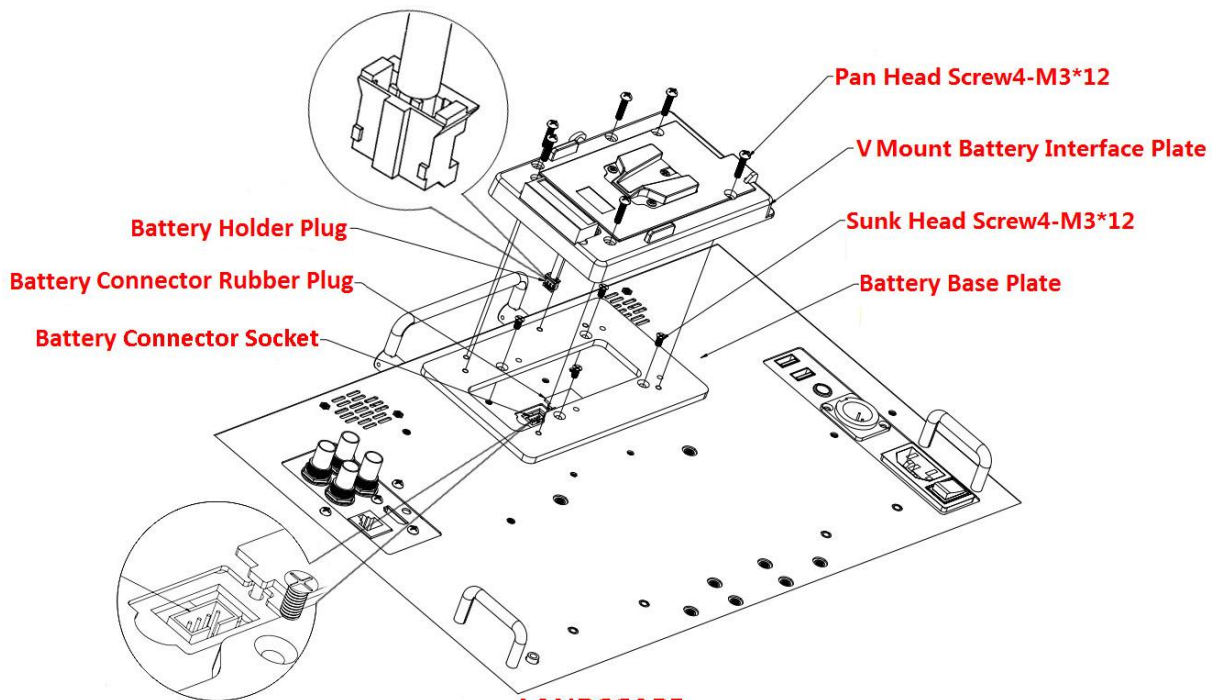
Figure 5.2-4 V-mount Battery Plate in Landscape
