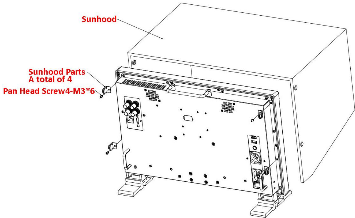
Figure 5.2-7 Mount a Sunhood for LCM-170E
