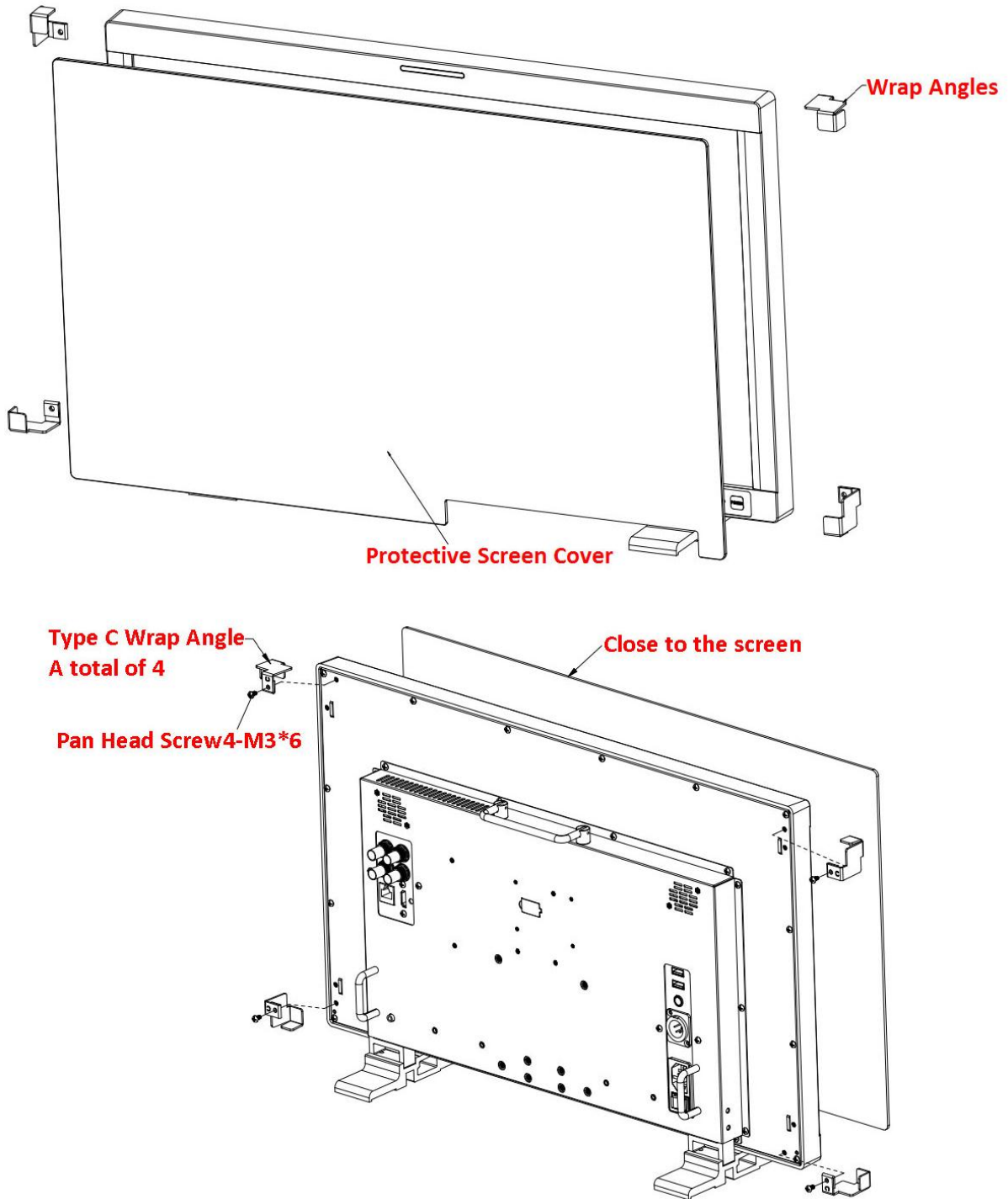
Figure 5.2-11 Mount a Protective Screen for LCM-230E
