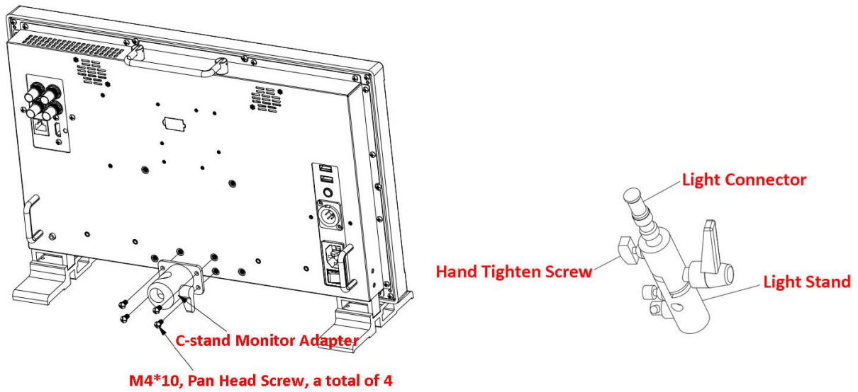
Figure 5.2-12 Adapter C-Stand to LCM-E Monitor
