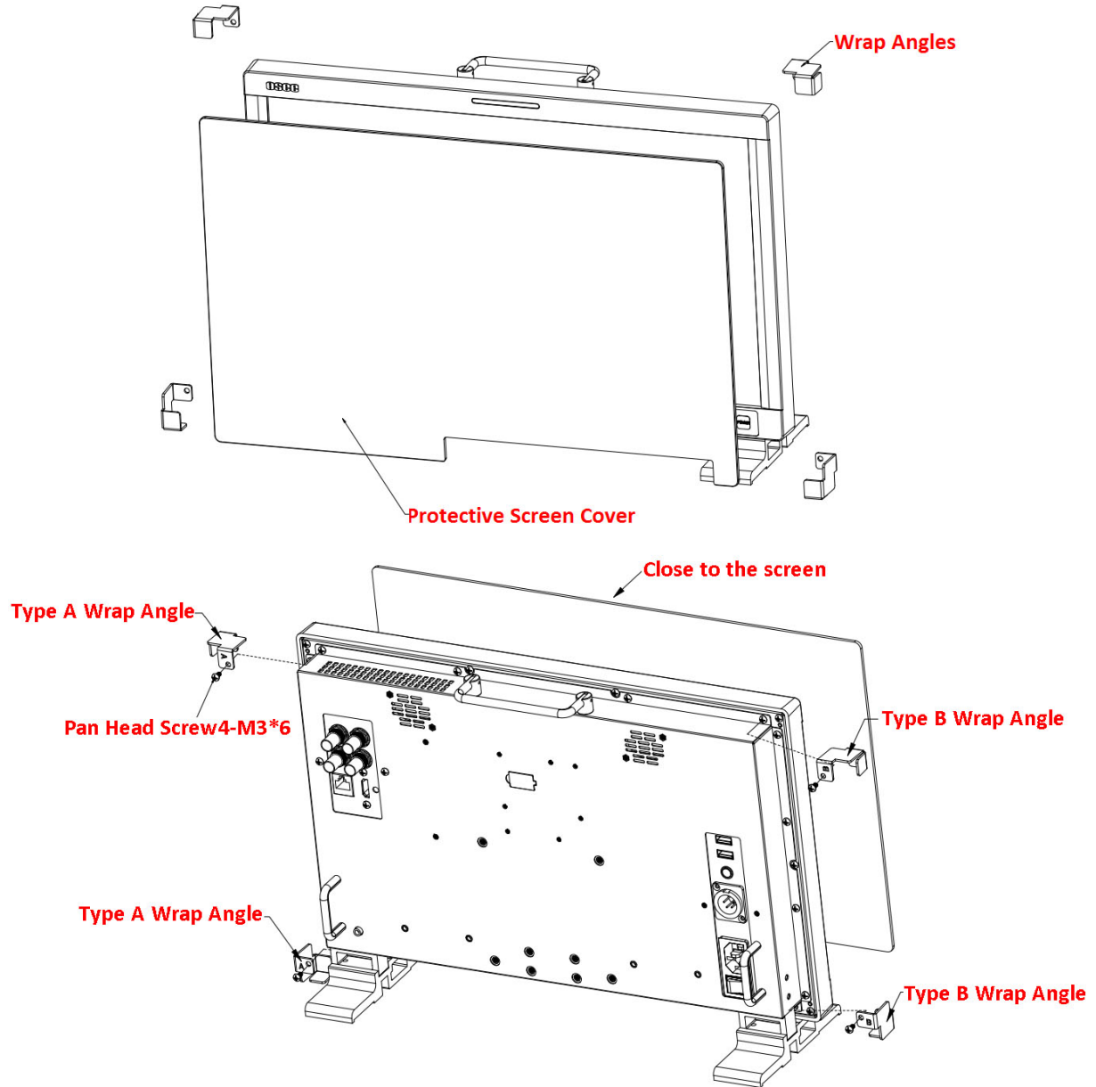
Figure 5.2-10 Mount a Protective Screen for LCM-170E
