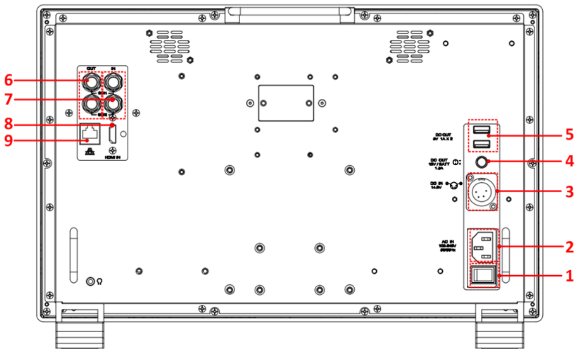
Figure 3.2-3 The Rear Panel of LCM170-E Monitor
