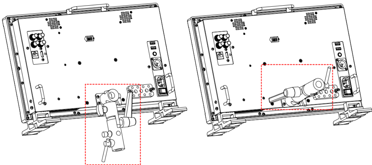
Figure 5.2-13 Connecting to Light Stand
