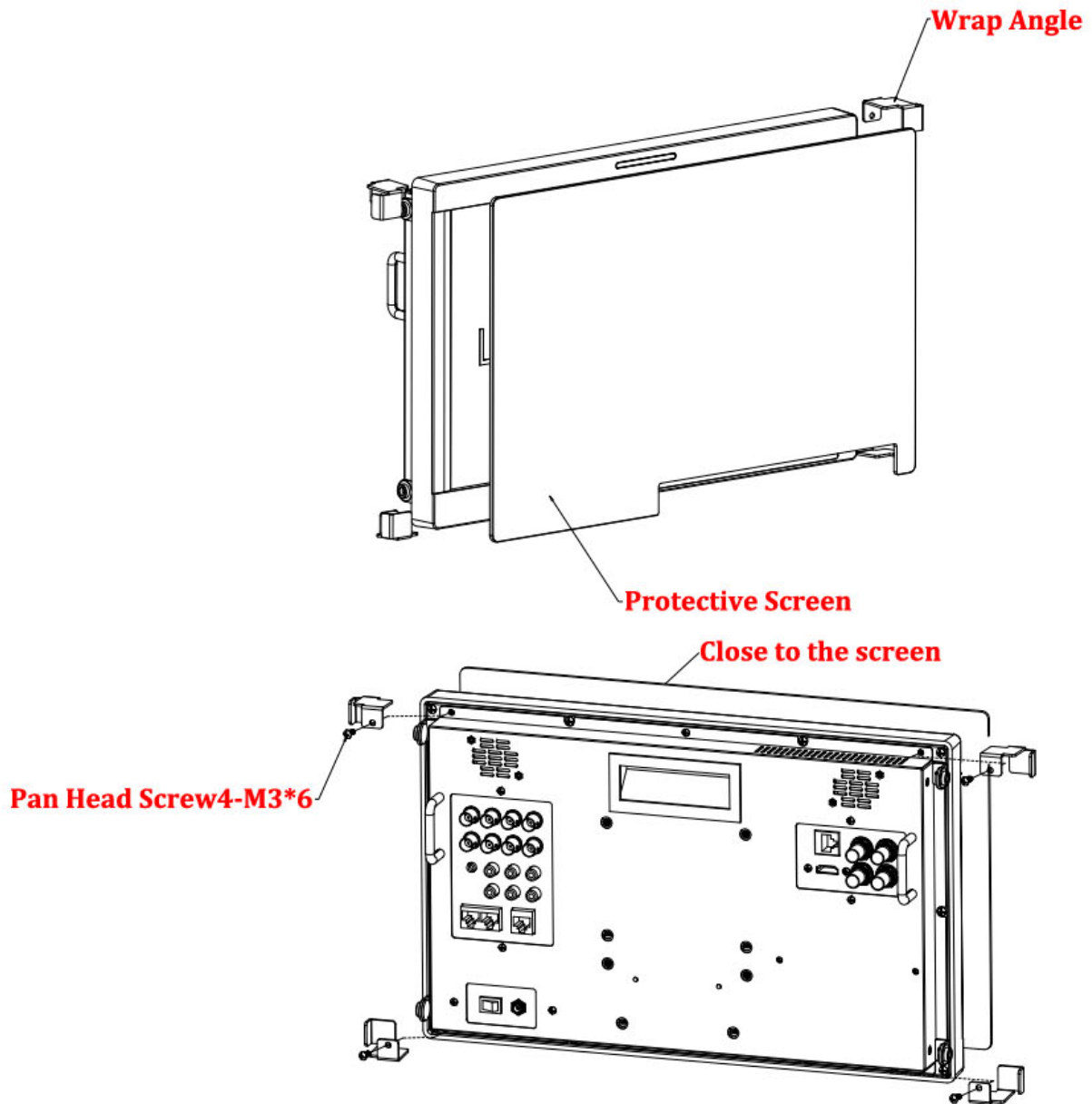
Figure 5.2-9 Mount a Protective Screen for LCM-156E
