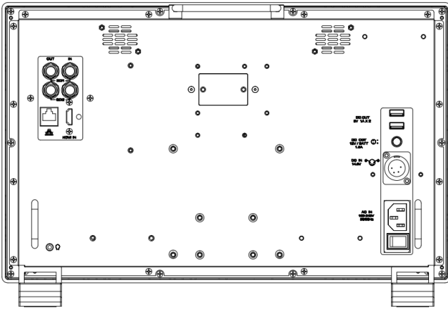
Rear Panel
