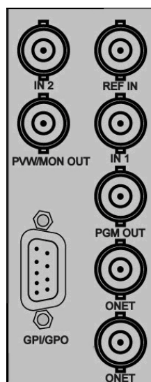
Fig.1-2 Back Connector of SAC6840N
