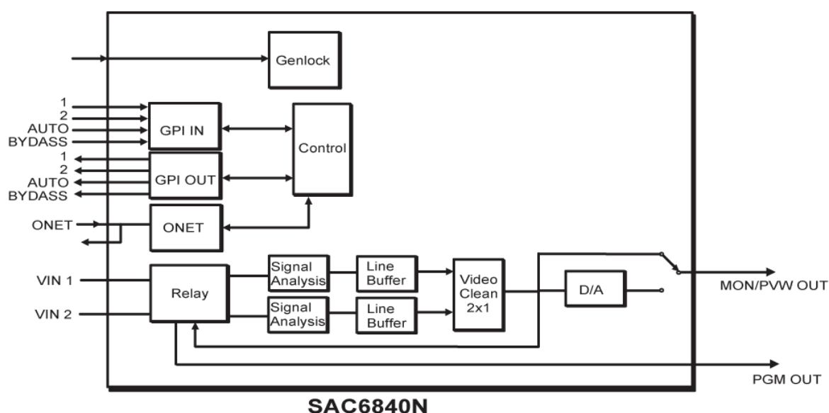
Fig. 1-3 Signal Flow of SAC6840N
