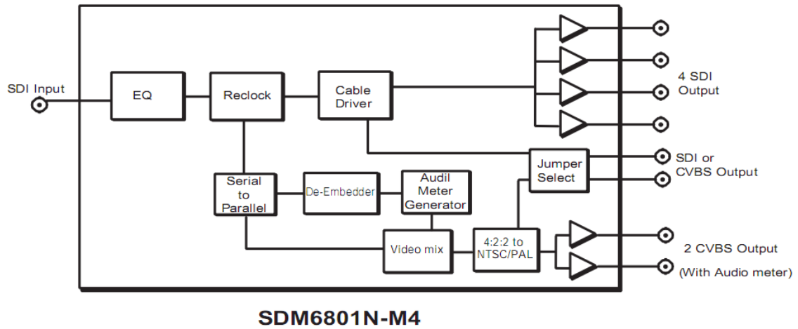
Figure 1-3 Basic signal flow of SDM6801N-M4
