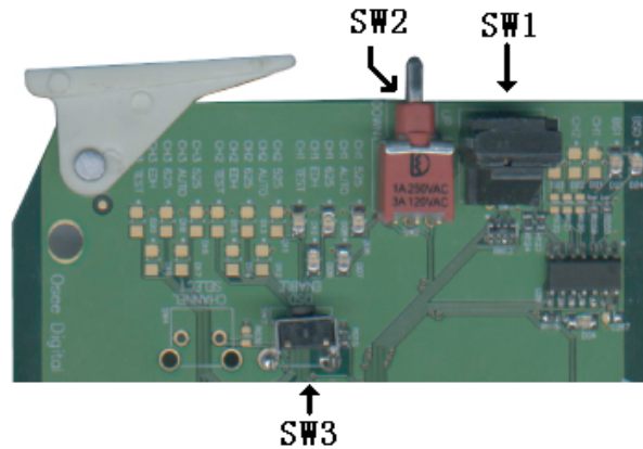
Figure 3-1 The Positions of SW1 SW2 and SW3
