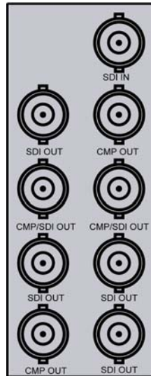
Figure 1-2 the Back Connector of SDM6801N-M4
