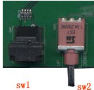
Figure 3-1 The Positions of SW1 SW2
