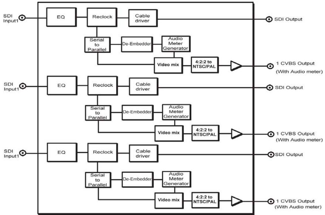
Figure 1-5 Basic signal flow of SDM6803N-M4
