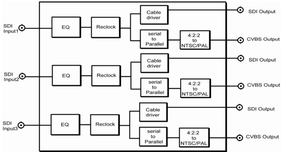
Figure 1-3 Basic signal flow of SDM6803N
