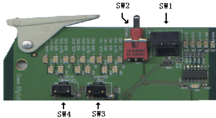
Figure 3-1 The Positions of SW1 SW2 SW3 and SW4
