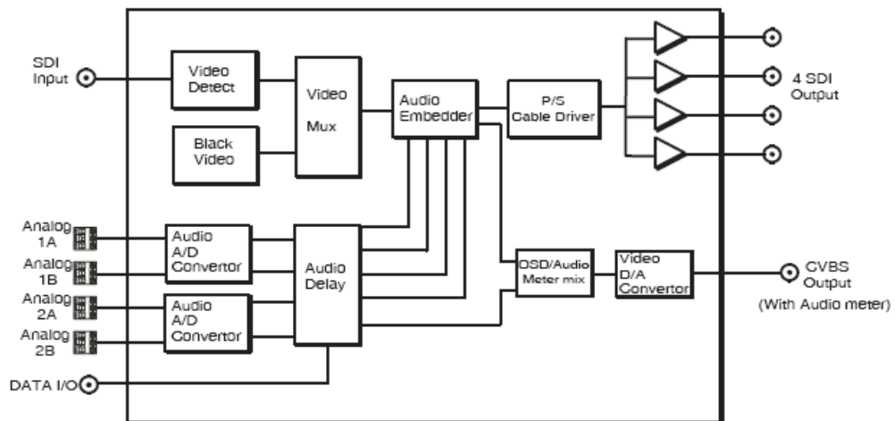
Fig. 1-4 Signal Flow of SMX6810NS
