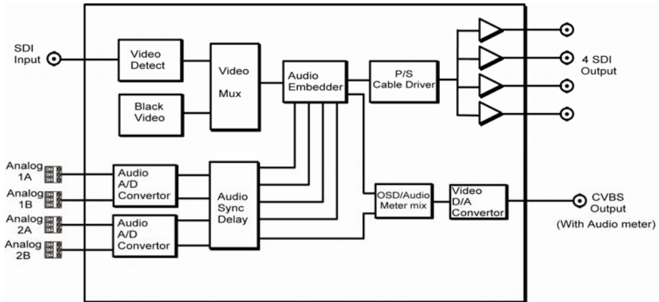
Fig. 1-3 Signal Flow of SMX6810N
