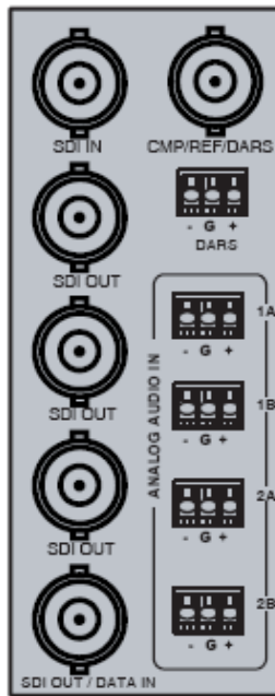
Fig.1-2 Back Connector of SMX6810N(S)
